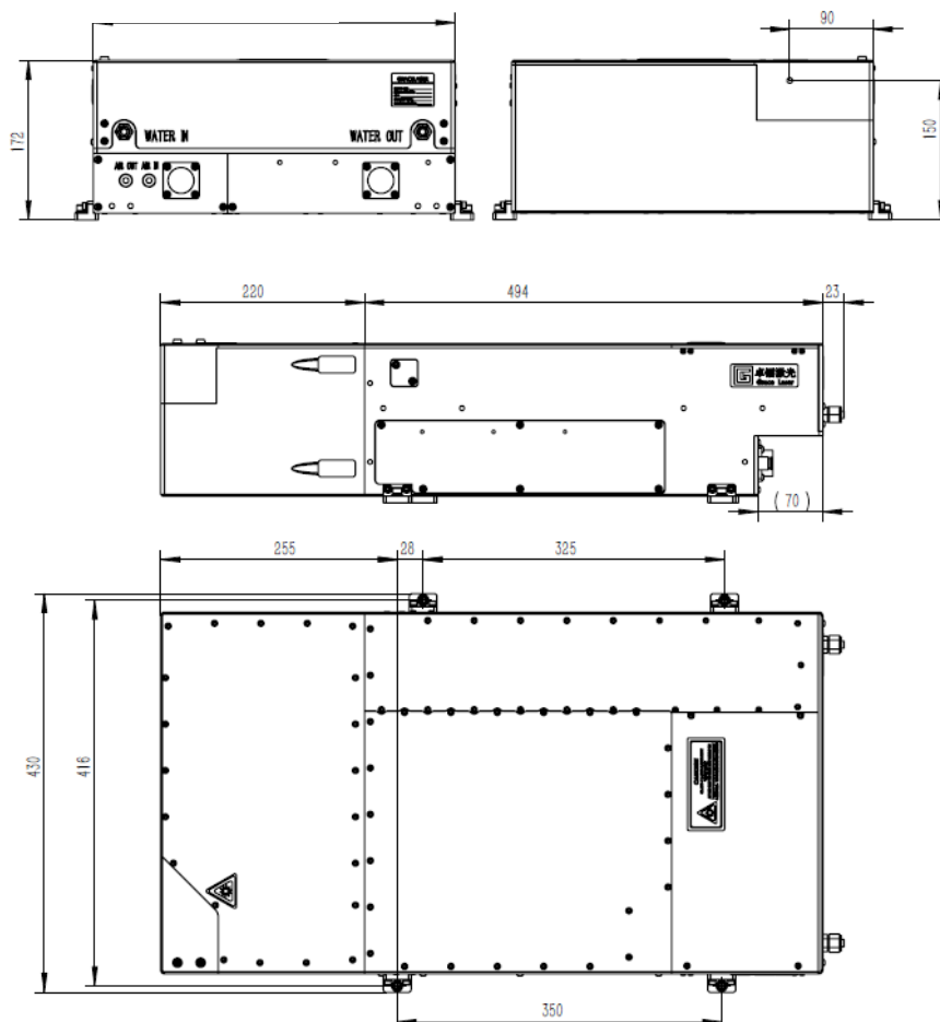
Genius-DUV laser head dimension Unit: mm
